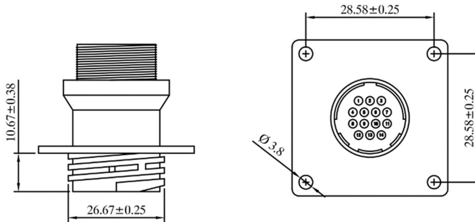
FIXED PART
